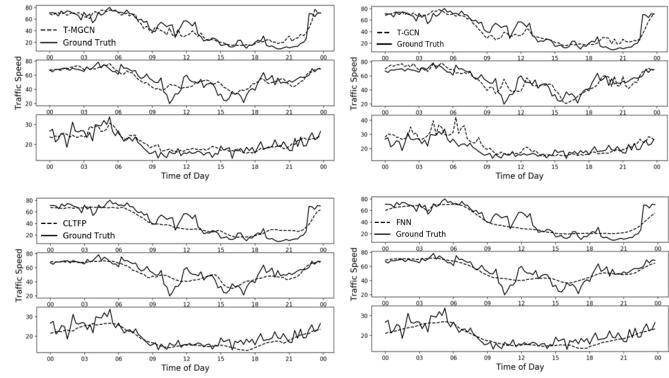
Fig. 8. A case study of traffic flow prediction: (a) prediction by T-MGCN; (b) prediction by T-GCN; (c) prediction by CLTFP; (d) prediction by FNN.
